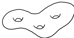
FIGURE 18.3. A genus 3 Riemann surface
