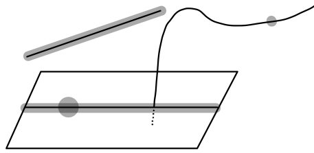
FIGURE 6.3. This scheme has six associated points, of which three are embedded points. A function is a zerodivisor if it vanishes at any of these six points.
