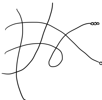
FIGURE 28.1. This curve has genus 8 (count the “holes”!)
