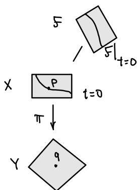
FIGURE 24.4. The (sufficient) slicing criterion for flatness on the source, Theorem 24.7.9
