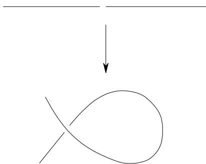
FIGURE 19.1. (variant of Figure 8.4) The projectivity hypothesis in Theorem 19.1.1 cannot be dropped
