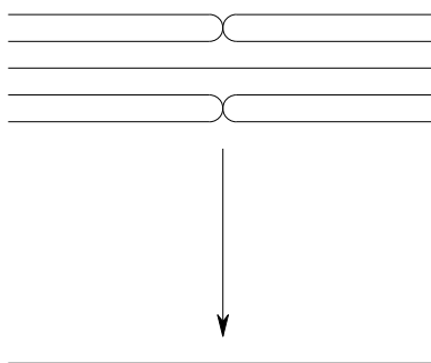
FIGURE 21.4. An example where the branch divisor appears with multiplicity 2 (see Exercise 21.4.C)
