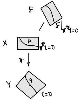
FIGURE 24.3. The (necessary and sufficient) slicing criterion for flatness on the target, Theorem 24.7.6
