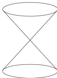
FIGURE 9.4. The cone x^2 + y^2 = z^2 in \mathbb{A}^3 .
