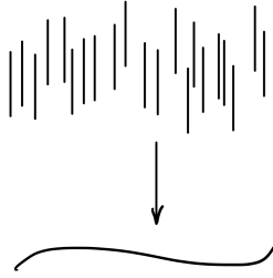
FIGURE 24.7. We don't want this to be a "smooth morphism"
