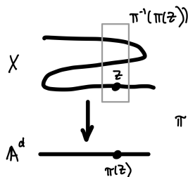
FIGURE 12.2. Key step in proof of Theorem 12.2.9
