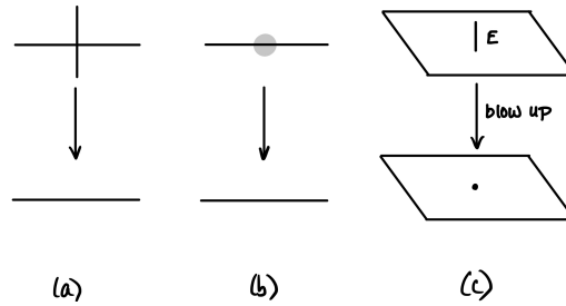
FIGURE 24.2. Morphisms that are not flat (Exercise 24.2.L)
