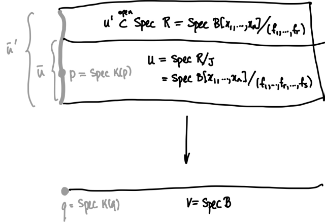
FIGURE 24.8. Geometry behind part of the proof of Theorem 24.9.8
