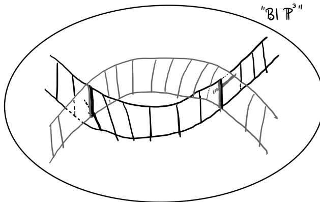
FIGURE 24.5. Hironaka's example of a proper nonprojective smooth threefold
