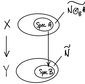
FIGURE 14.1. The pullback of a quasicoherent sheaf (module-theoretically)
