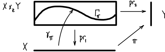
FIGURE 11.2. The graph morphism
