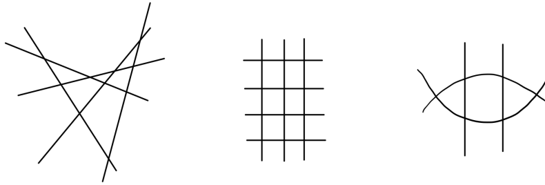
FIGURE 30.2. These curves have arithmetic genus 6, 6, and 3 respectively
