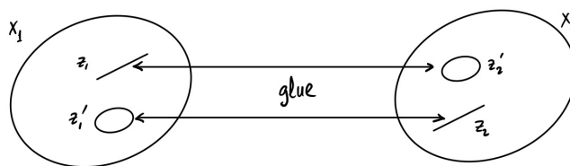
FIGURE 17.2. Building a proper nonprojective variety
