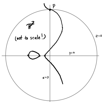
FIGURE 20.5. Finding the Weierstrass cubic incarnation of an elliptic curve
