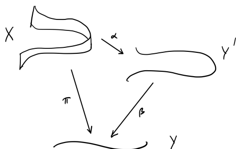
FIGURE 30.4. Stein Factorization
