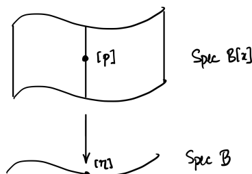
FIGURE 13.4. The geometry behind the proof of Proposition 13.3.6
