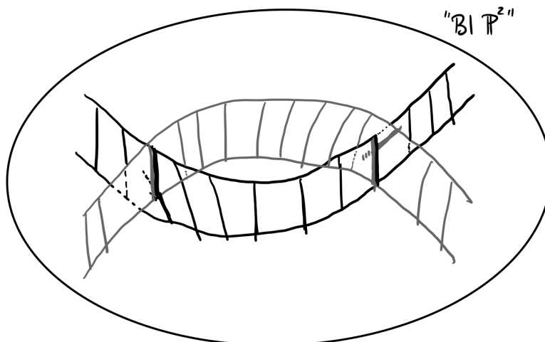
FIGURE 25.3. Hironaka's example of a proper nonprojective smooth threefold
