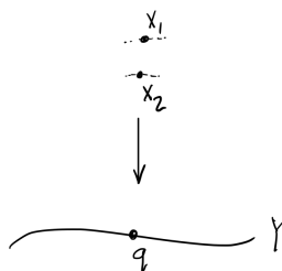
FIGURE 30.3. “Formal neighborhoods” of X_1 and X_2 in the proof of Zariski’s Connectedness Lemma 30.5.1
