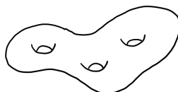
FIGURE 19.2. A genus 3 Riemann surface
