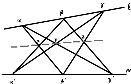
FIGURE 20.2. Pappus' Theorem
