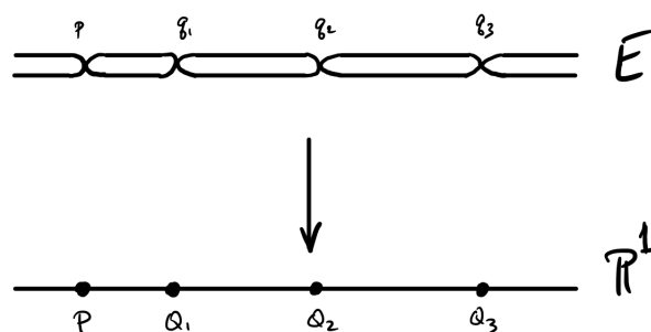
FIGURE 20.4. Elliptic curves yield double covers of the projective line, branched at four points (§20.9.5)
