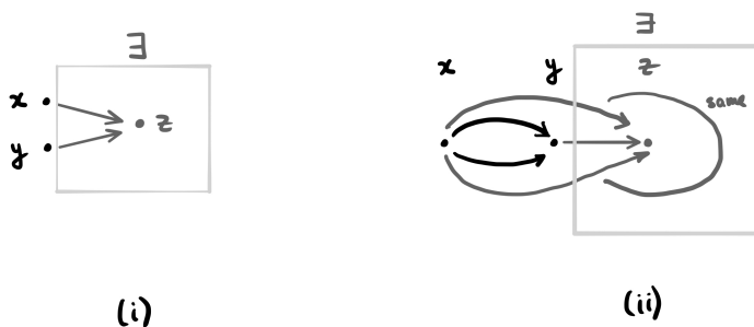
FIGURE 1.1. A filtered category (pictorial definition)
