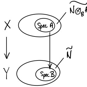
FIGURE 17.1. The pullback of a quasicoherent sheaf (module-theoretically)
