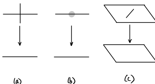
FIGURE 25.2. Morphisms that are not flat (Exercise 25.2.K)
