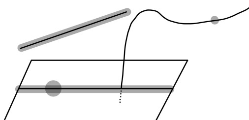
FIGURE 6.1. This scheme has six associated points, of which three are embedded points. A function is a zerodivisor if it vanishes at any of these six points.
