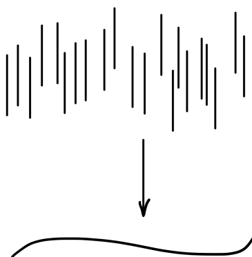
FIGURE 26.2. We don't want this to be a "smooth morphism"
