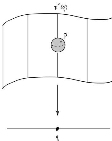
FIGURE 12.3. Exercise 12.4.A: the codimension of a point in the total space is bounded by the sum of the codimension of the point in the fiber plus the codimension of the image in the target
