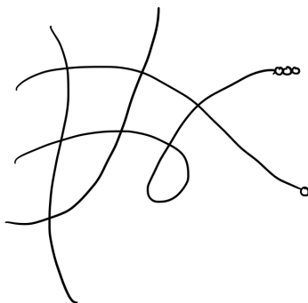
FIGURE 30.1. This curve has genus 8 (count the “holes”!)
