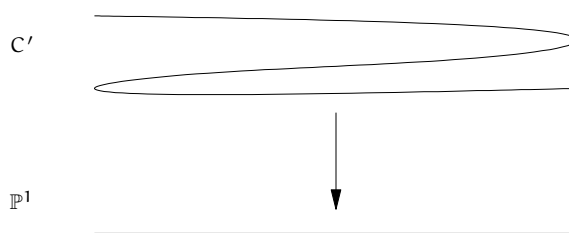
FIGURE 18.1. Constructing a projective regular model of a curve C over k via a finite cover of \mathbb{P}^1
