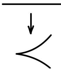
FIGURE 10.4. Normalization of a cusp
