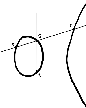
FIGURE 20.7. The group law on the elliptic curve, geometrically
