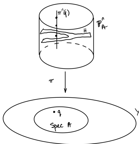
FIGURE 19.1. The key construction in the proof of Theorem 19.1.7
