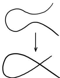
FIGURE 8.4. The “normalization” of the nodal cubic \text{Spec } k[t] \rightarrow \text{Spec } k[x, y]/(y^2 - x^2 - x^3) given by (x, y) \mapsto (t^2 - 1, t^3 - t) is finite
