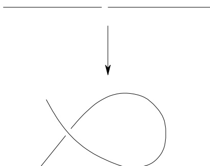
FIGURE 20.1. (variant of Figure 8.4) The projectivity hypothesis in Theorem 20.1.1 cannot be dropped
