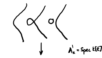
FIGURE 25.1. A flat family of smooth curves degenerating to a nodal curve: y^2 = x^3 + x^2 + tx .
