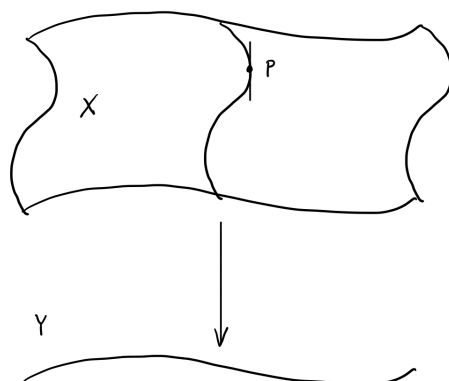
FIGURE 22.1. The relative tangent space of a morphism X \rightarrow Y at a point p
