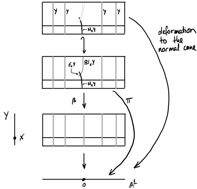
FIGURE 23.3. Deformation to the normal cone (§23.4.17)
