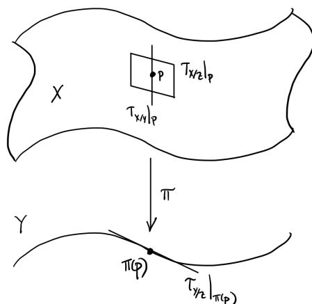
FIGURE 22.2. A sketch of the geometry behind the cotangent exact sequence
