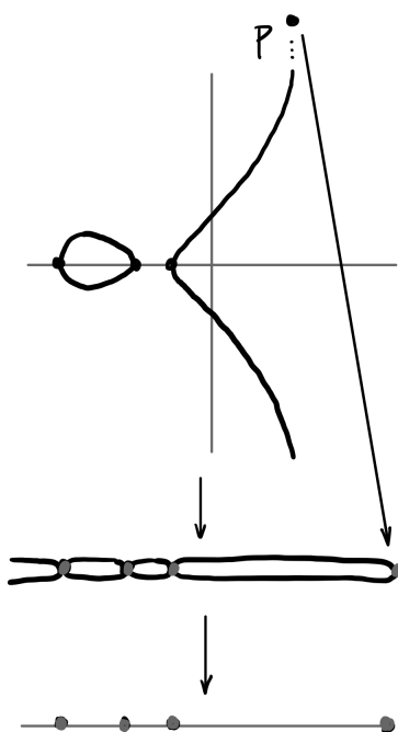
FIGURE 20.6. From the Weierstrass cubic to the double cover interpretation of an elliptic curve (cf. Figure 20.5)
