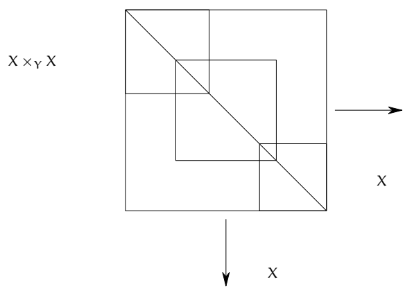
FIGURE 11.1. An open neighborhood of the diagonal is covered by U_{ij} \times_{V_i} U_{ij}
