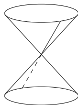
FIGURE 13.1. V(x, z) \subset \text{Spec } k[x, y, z]/(xy - z^2) is a line on a cone
