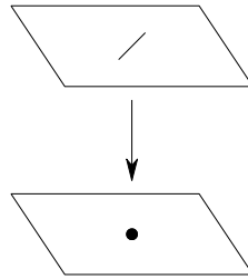
FIGURE 10.3. A first example of a blow-up
