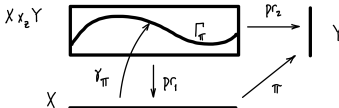
FIGURE 11.2. The graph morphism
