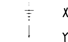
FIGURE 9.5. Yuck (Example 4 of Definition 9.4.2)
