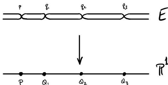
FIGURE 19.4. Elliptic curves yield double covers of the projective line, branched at four points (§19.9.5)
