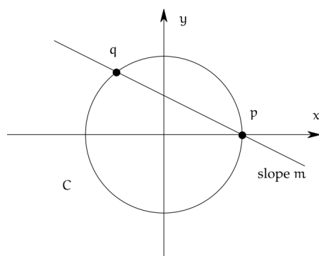
FIGURE 7.2. Finding primitive Pythagorean triples using geometry
