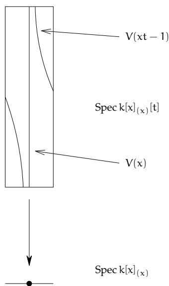
FIGURE 12.3. Dimension and codimension behave oddly on the surface \text{Spec } k[x]_{(x)}[t]
