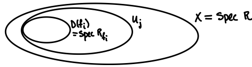
FIGURE 18.2. The final step in the proof of Theorem 18.2.2
