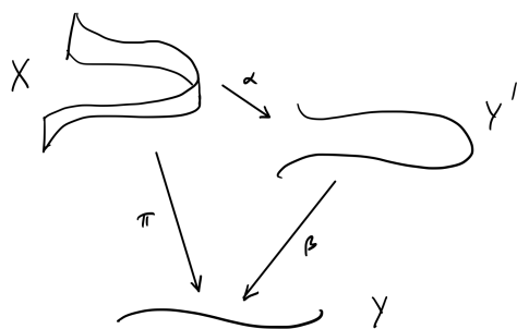
FIGURE 29.4. Stein Factorization
