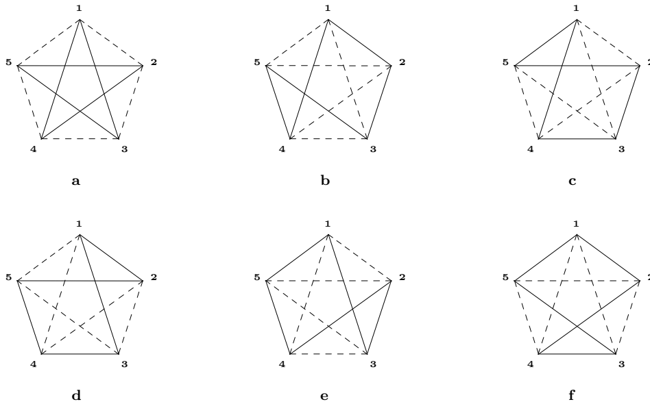
FIGURE 1. The six mystic pentagons, with black and white (dashed) edges
