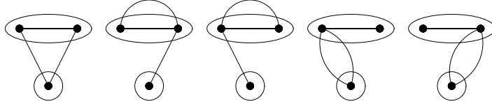
FIGURE 1. Counting T_\alpha^1 = 4 when \alpha is the partition 3 = 1 + 2 (the last two both count with multiplicity 1/2 )
