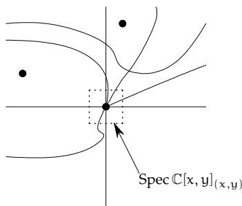
FIGURE 4.5. Picturing \text{Spec } \mathbb{C}[x, y]_{(x, y)} as a “shred of A^2_{\mathbb{C}} ”. Only those points near the origin remain.
