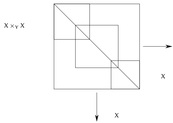
FIGURE 10.1. an open neighborhood of the diagonal is covered by \mathcal{U}_{ij} \times_{V_i} \mathcal{U}_{ij}
