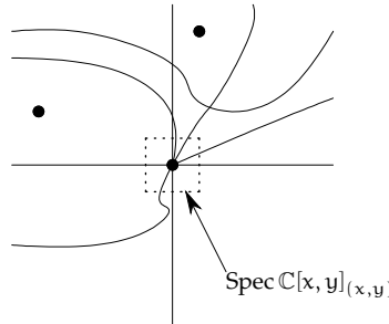
FIGURE 3.5. Picturing \text{Spec } \mathbb{C}[x, y]_{(x, y)} as a “shred of \mathbb{A}_{\mathbb{C}}^2 ”. Only those points near the origin remain.
