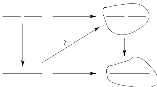
FIGURE 13.4. The valuative criterion for separatedness
