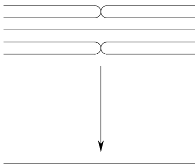
FIGURE 22.4. An example where the branch divisor appears with multiplicity 2 (see Exercise 22.5.C)
