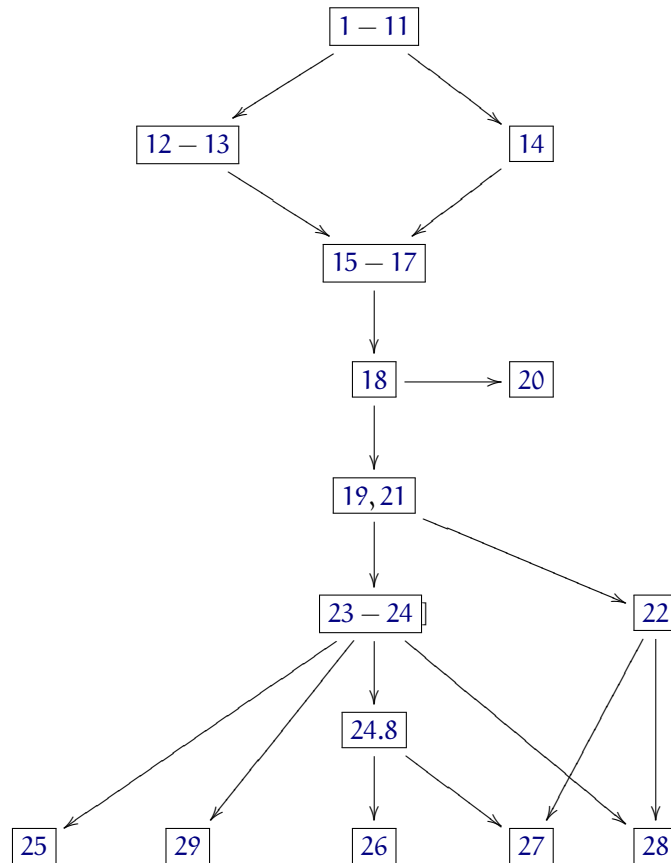
FIGURE 0.1. Important logical dependencies among chapters (or more precisely, a directed graph showing which chapter should be read before which other chapter)
