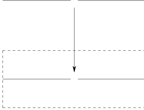
FIGURE 9.1. The locally closed embedding \operatorname{Spec} k[t, t^{-1}] \rightarrow \operatorname{Spec} k[x, y] ( t \mapsto (t, 0) = (x, y) , i.e., (x, y) \rightarrow (t, 0) )
