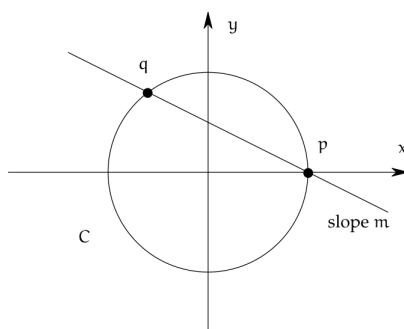
FIGURE 7.2. Finding primitive Pythagorean triples using geometry
