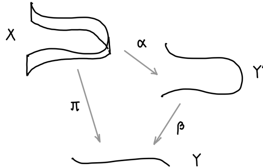
FIGURE 28.4. Stein Factorization
