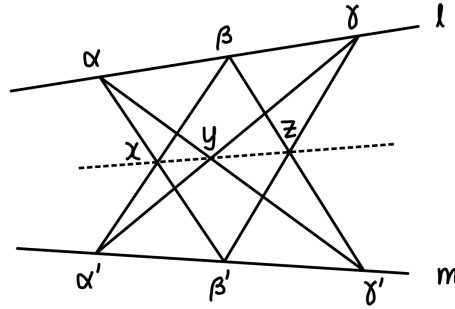
FIGURE 19.2. Pappus' Theorem
