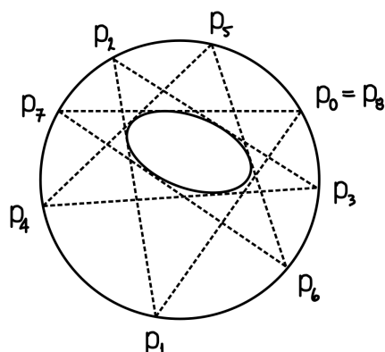
FIGURE 19.8. Poncelet's Porism 19.10.8
