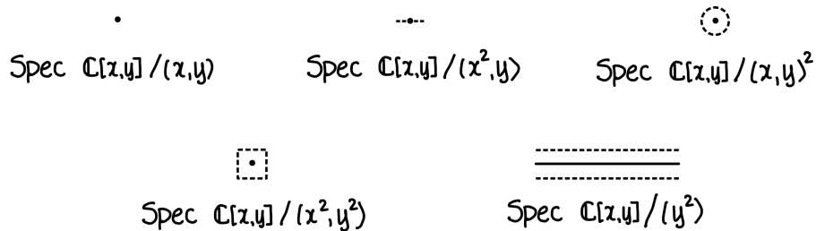
FIGURE 4.3. Picturing quotients of \mathbb{C}[x, y]
