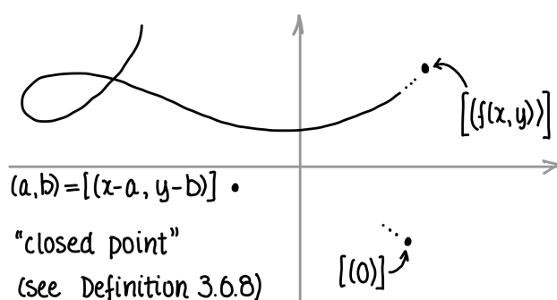
FIGURE 3.3. Picturing \mathbb{A}_{\mathbb{C}}^2 = \text{Spec } \mathbb{C}[x, y]
