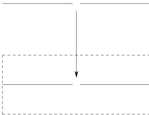
FIGURE 9.1. The locally closed immersion \operatorname{Spec} k[t, t^{-1}] \rightarrow \operatorname{Spec} k[x, y] (t \mapsto (t, 0) = (x, y), \text{ i.e. } (x, y) \mapsto (t, 0))
