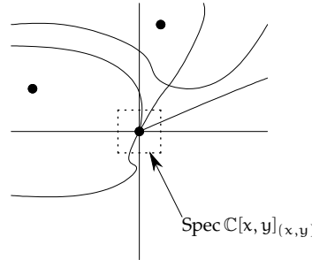
FIGURE 3.5. Picturing \text{Spec } \mathbb{C}[x, y]_{(x, y)} as a “shred of A_{\mathbb{C}}^2 ”. Only those points near the origin remain.
