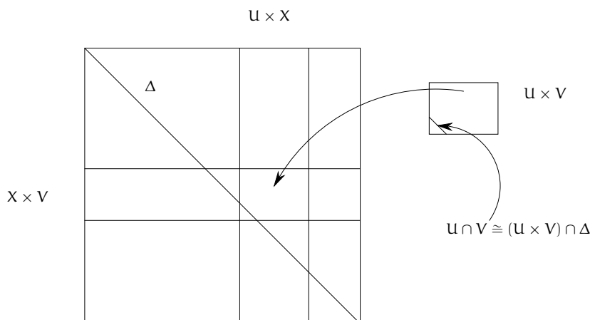
FIGURE 11.2. Small Proposition 11.1.6
