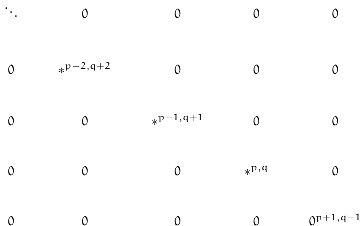
FIGURE 2.1. A (p, q) -strip (in S^{p, q} \subset \mathbb{E}^{p+q} ). Clearly S^{0, k} = \mathbb{E}^k .
