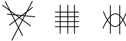
FIGURE 28.2. These curves have arithmetic genus 6, 6, and 3 respectively
