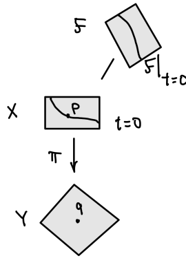
FIGURE 24.4. The (sufficient) slicing criterion for flatness on the source, Theorem 24.7.9
