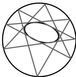
FIGURE 19.8. Poncelet's Porism 19.10.8
