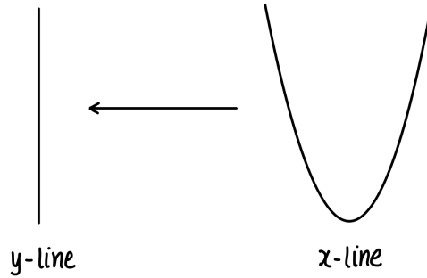
FIGURE 3.6. The map \mathbb{C} \rightarrow \mathbb{C} given by x \mapsto y = x^2
