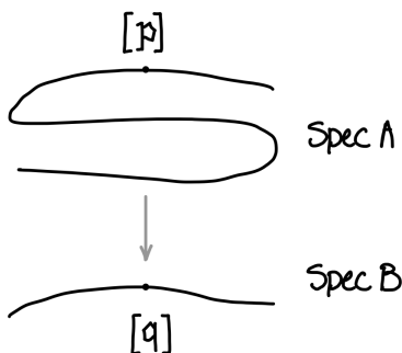
FIGURE 8.1. A picture of the Lying Over Theorem 8.2.5: if \phi: B \rightarrow A is an integral extension, then \text{Spec } A \rightarrow \text{Spec } B is surjective
