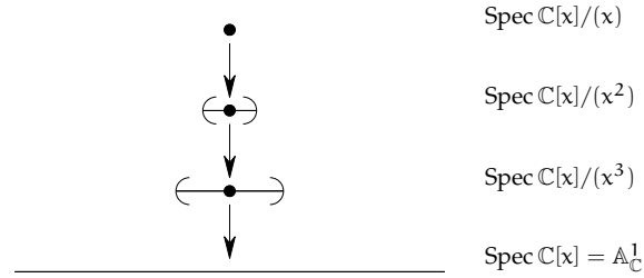
FIGURE 4.2. Picturing quotients of \mathbb{C}[x]
