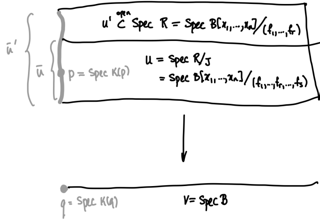
FIGURE 24.8. Geometry behind part of the proof of Theorem 24.9.8
