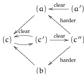
FIGURE 17.3. Structure of the proof of Theorem 17.6.2, up to the last step
