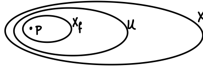
FIGURE 17.4. Visual aid for the proof of Theorem 17.6.2
