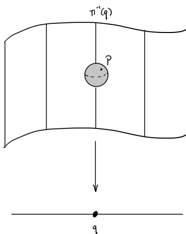
FIGURE 12.4. Exercise 12.5.A: the codimension of a point in the total space is bounded by the sum of the codimension of the point in the fiber plus the codimension of the image in the target
