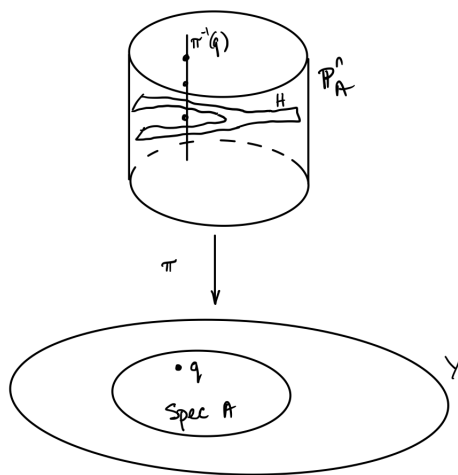
FIGURE 19.1. The key construction in the proof of Theorem 19.1.6
