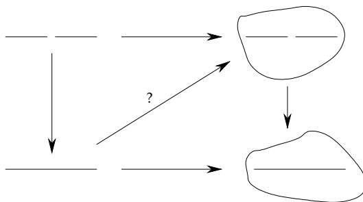
FIGURE 13.5. The valuative criterion for separatedness
