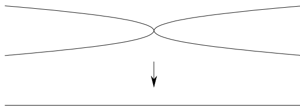
FIGURE 10.2. The map \mathbb{C} \rightarrow \mathbb{C} given by y \mapsto y^2
