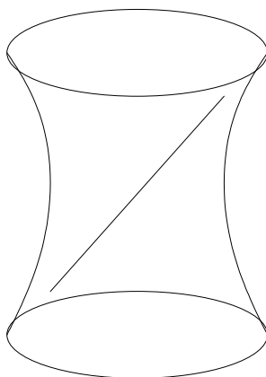
FIGURE 13.2. The line V(x, z) on the smooth quadric surface V(wz - xy) \subset \mathbb{P}^3 .
