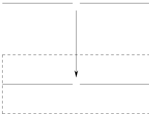
FIGURE 9.1. The locally closed embedding \text{Spec } k[t, t^{-1}] \rightarrow \text{Spec } k[x, y] ( t \mapsto (t, 0) = (x, y) , i.e. (x, y) \mapsto (t, 0) )
