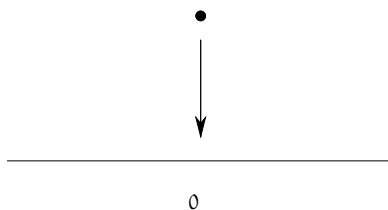
FIGURE 8.3. The “closed immersion” \text{Spec } k \rightarrow \text{Spec } k[t] given by t \mapsto 0 is finite
