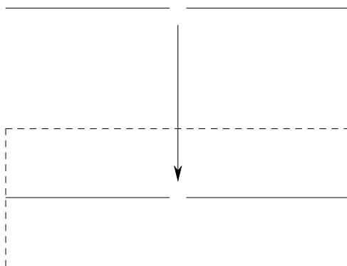
FIGURE 9.1. The locally closed immersion \mathrm{Spec} k[t, t^{-1}] \rightarrow \mathrm{Spec} k[x, y] \ (t \mapsto (t, 0) = (x, y), \text{ i.e. } (x, y) \rightarrow (t, 0))
