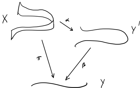
FIGURE 30.4. Stein Factorization
