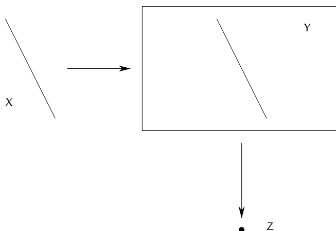
FIGURE 23.3. A sketch of the geometry behind the conormal exact sequence
