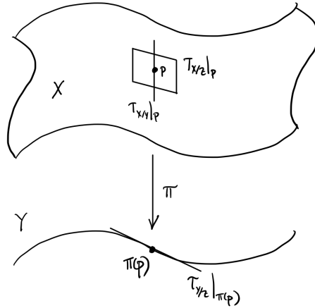
FIGURE 21.2. The geometry behind the cotangent exact sequence
