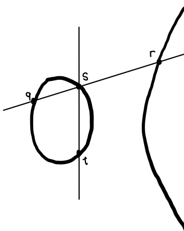
FIGURE 19.7. The group law on the elliptic curve, geometrically
