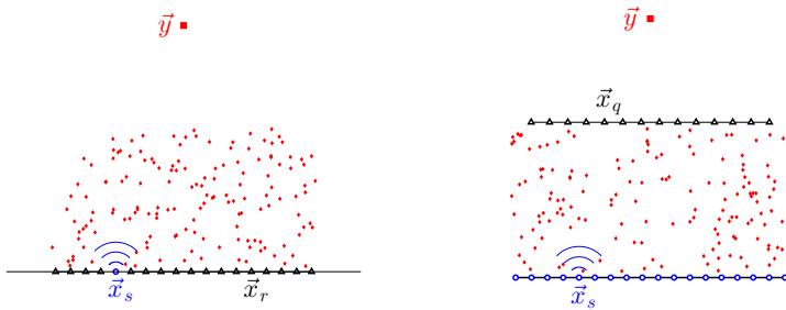
FIG. 1.1. Sensor array imaging of a reflector located at \vec{y} through a scattering medium. Left: Conventional imaging, \vec{x}_s is a source, \vec{x}_r is a receiver. Right: Use of an auxiliary passive array for imaging through a scattering medium, \vec{x}_s is a source, \vec{x}_q is a receiver located beyond the scattering medium.
