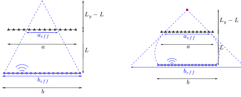
FIG. 2.1. If the medium is homogeneous (left picture), the illumination cone is determined by the physical source array diameter b_{\text{eff}} = b . In the random paraxial regime (right picture), the angular diversity of the waves that illuminate the reflector is increased by scattering and the effective illumination cone is enhanced and corresponds to an effective source array diameter b_{\text{eff}} > b .
