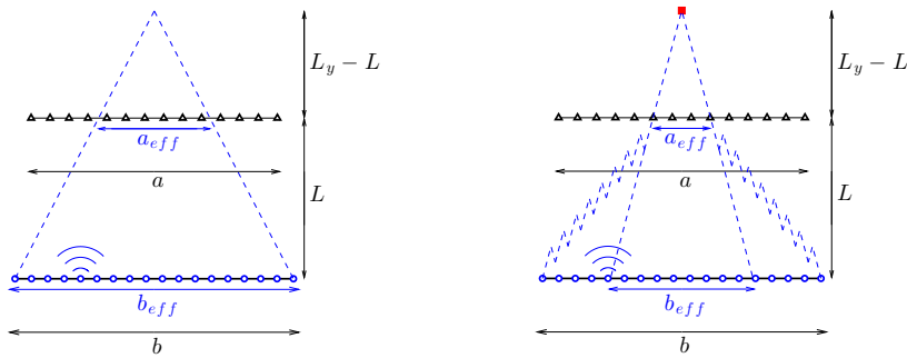
FIG. 2.2. If the medium is homogeneous (left picture), the illumination cone is determined by the physical source array diameter b_{\text{eff}} = b . If the medium is randomly layered (right picture), the angular diversity of the waves that illuminate the reflector is reduced by scattering (only the waves with wavevectors close to the vertical direction can reach the reflector after multiple scattering events that conserve the wavevectors in the layered case) and the effective illumination cone is reduced and corresponds to an effective source array diameter b_{\text{eff}} < b .
