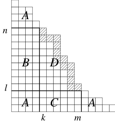
FIGURE 1. Unshaded boxes correspond to the partition \lambda . Shaded boxes correspond to the border strip \mu - \lambda .
