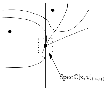
FIGURE 3.5. Picturing \text{Spec } \mathbb{C}[x, y]_{(x, y)} as a “shred of A_{\mathbb{C}}^2 ”. Only those points near the origin remain.
