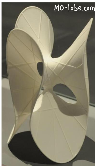
FIGURE 27.1. Twenty-seven lines on a cubic surface
