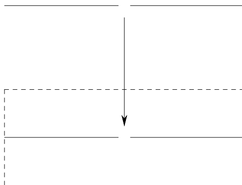
FIGURE 8.1. The locally closed embedding \text{Spec } k[t, t^{-1}] \rightarrow \text{Spec } k[x, y] ( t \mapsto (t, 0) = (x, y) , i.e., (x, y) \rightarrow (t, 0) )
