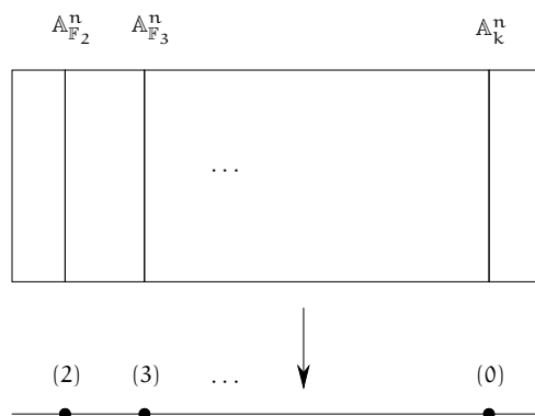
FIGURE 3.7. A picture of \mathbb{A}_{\mathbb{Z}}^n \rightarrow \text{Spec } \mathbb{Z} as a “family of \mathbb{A}^n ’s”, or an “ \mathbb{A}^n -bundle over \text{Spec } \mathbb{Z} ”. What is k ?
