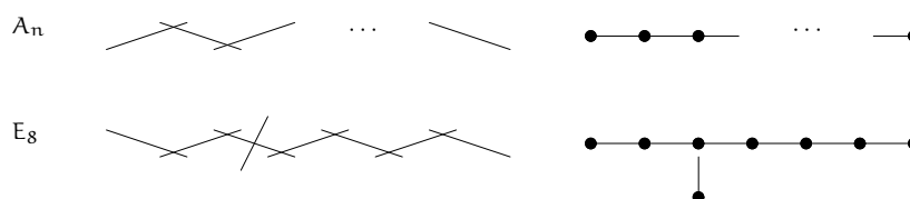
FIGURE 23.2. The exceptional divisors for resolutions of some ADE surface singularities, and their corresponding dual graphs (see Remark 23.4.5)
