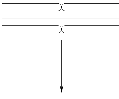
FIGURE 22.4. An example where the branch divisor appears with multiplicity 2 (see Exercise 22.7.C)
