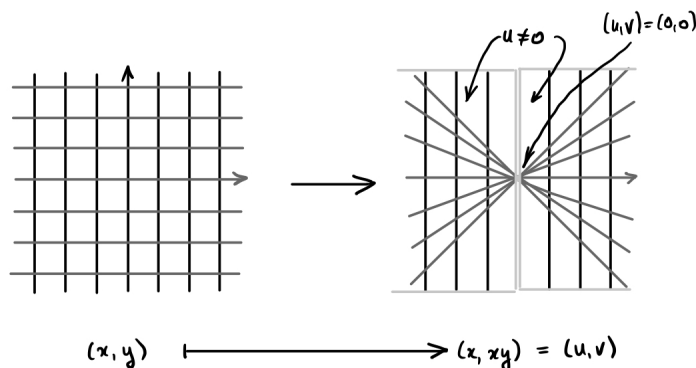
FIGURE 8.6. The image of (x, y) \mapsto (x, xy) = (u, v) .
