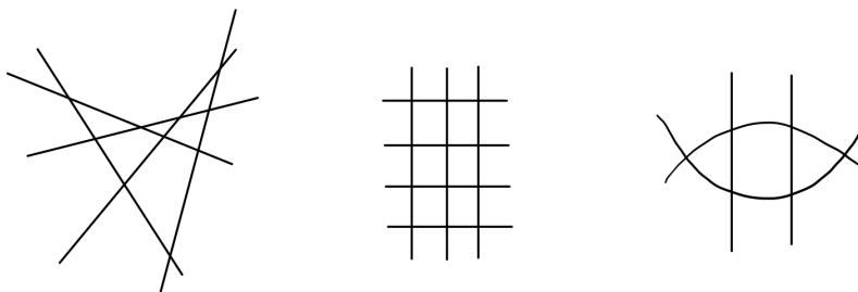
FIGURE 28.2. These curves have arithmetic genus 6, 6, and 3 respectively
