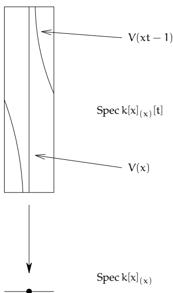
FIGURE 12.3. Dimension and codimension behave oddly on the surface \text{Spec } k[x]_{(x)}[t]
