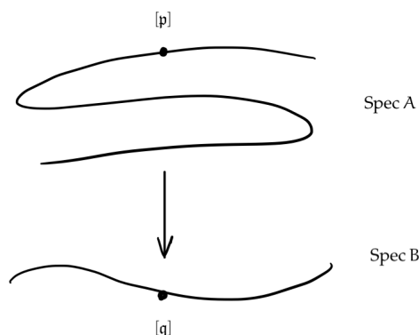
FIGURE 8.1. A picture of the Lying Over Theorem 8.2.5: if \phi: B \rightarrow A is an integral extension, then \text{Spec } A \rightarrow \text{Spec } B is surjective
