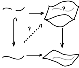
FIGURE 13.6. The valuative criterion for separatedness
