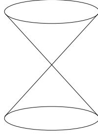
FIGURE 9.4. The cone x^2 + y^2 = z^2 .
