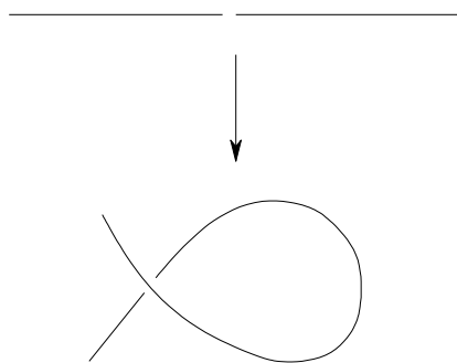
FIGURE 19.1. (variant of Figure 8.4) The projectivity hypothesis in Theorem 19.1.1 cannot be dropped
