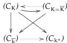
FIGURE 10.4. Connectedness conditions that will later turn out to be equivalent (solid arrows are trivial, dotted arrows are Exercise 10.5.F)
