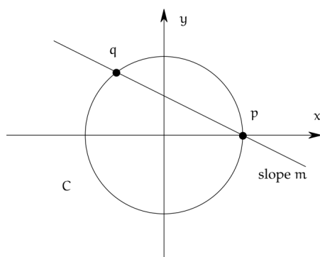
FIGURE 7.2. Finding primitive Pythagorean triples using geometry
