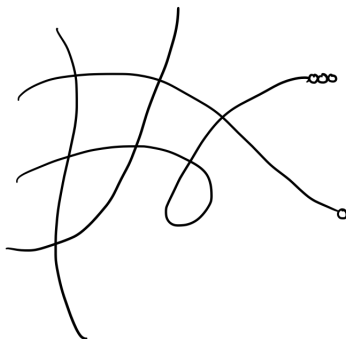
FIGURE 28.1. This curve has genus 8 (count the “holes”!)
