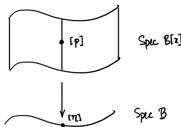
FIGURE 13.4. The geometry behind the proof of Proposition 13.3.7
