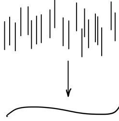
FIGURE 24.5. We don't want this to be a "smooth morphism"
