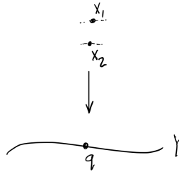
FIGURE 28.3. “Formal neighborhoods” of X_1 and X_2 in the proof of Zariski’s Connectedness Lemma 28.5.1
