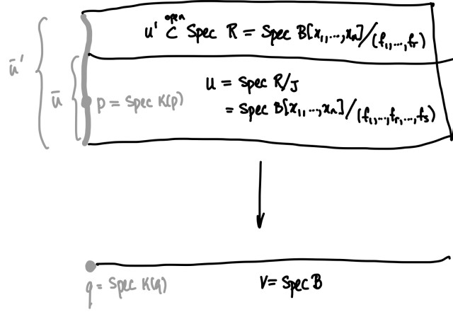
FIGURE 24.6. Geometry behind part of the proof of Theorem 24.8.8
