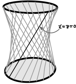
FIGURE 13.2. The line V(x, z) on the smooth quadric surface V(wz - xy) \subset \mathbb{P}^3 .
