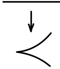
FIGURE 10.5. Normalization of a cusp
