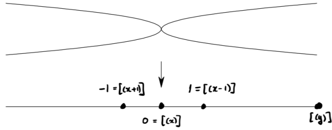
FIGURE 10.2. The map \mathbb{C} \rightarrow \mathbb{C} given by y \mapsto y^2
