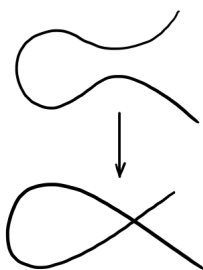
FIGURE 8.4. The “normalization” of the nodal cubic \text{Spec } k[t] \rightarrow \text{Spec } k[x, y]/(y^2 - x^2 - x^3) given by (x, y) \mapsto (t^2 - 1, t^3 - t) is finite
