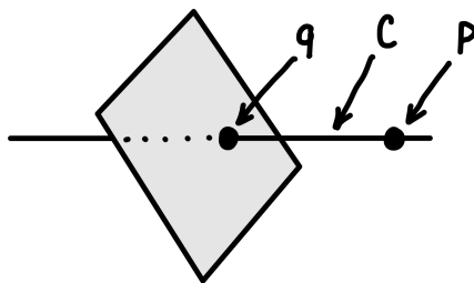
FIGURE 12.1. Behavior of codimension
