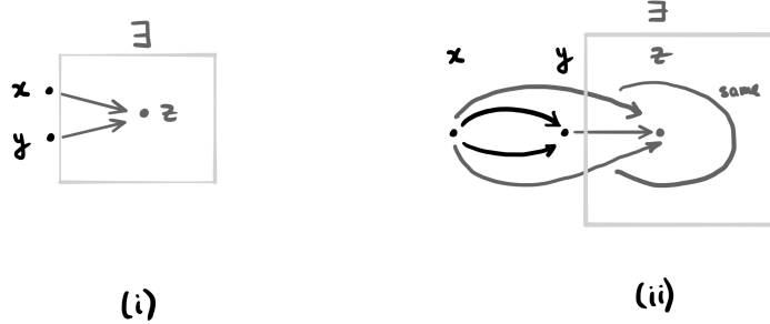
FIGURE 1.1. A filtered category (pictorial definition)
