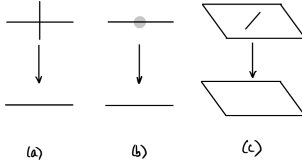
FIGURE 24.2. Morphisms that are not flat (Exercise 24.2.K)
