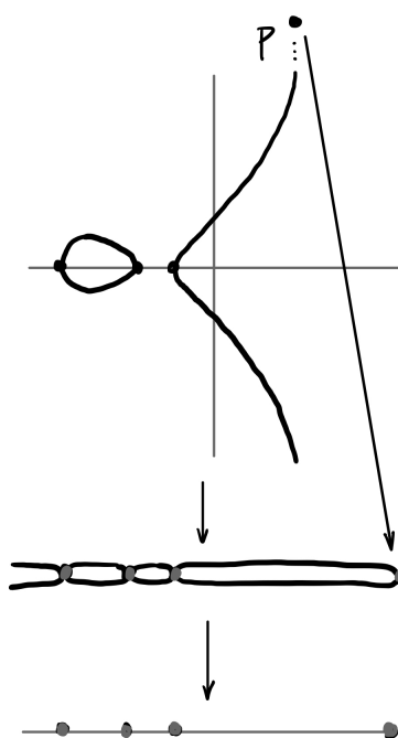
FIGURE 19.6. From the Weierstrass cubic to the double cover interpretation of an elliptic curve (cf. Figure 19.5)
