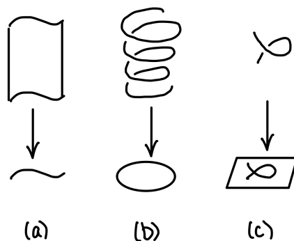
FIGURE 24.4. Sketches of notions from differential geometry: (a) maps “locally on the source a smooth fibration”, (b) local isomorphisms, and (c) immersions. (In algebraic geometry: (a) smooth morphisms, (b) étale morphisms, and (c) unramified morphisms.)
