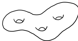
FIGURE 18.3. A genus 3 Riemann surface
