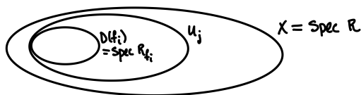
FIGURE 18.2. The final step in the proof of Theorem 18.2.2
