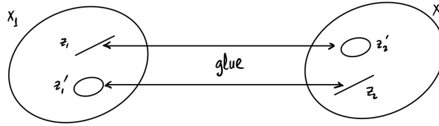
FIGURE 15.1. Building a proper nonprojective variety
