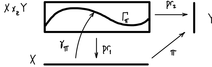
FIGURE 11.2. The graph morphism
