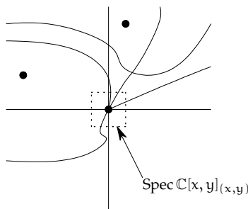
FIGURE 3.5. Picturing \text{Spec } \mathbb{C}[x, y]_{(x, y)} as a “shred of \mathbb{A}^2_{\mathbb{C}} ”. Only those points near the origin remain.
