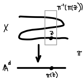
FIGURE 12.2. Key step in proof of Theorem 12.2.9
