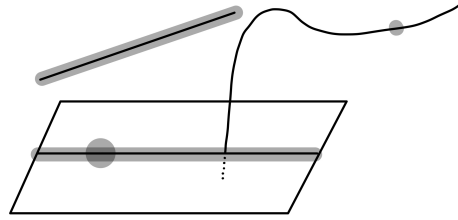
FIGURE 6.3. This scheme has six associated points, of which three are embedded points. A function is a zerodivisor if it vanishes at any of these six points.
