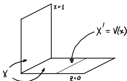
FIGURE 9.6. Order matters in a regular sequence (in the “non-local” situation), for silly reasons
