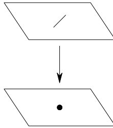
FIGURE 10.3. A first example of a blow-up
