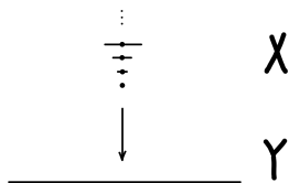
FIGURE 9.5. Yuck (Example 4 of Definition 9.4.2)
