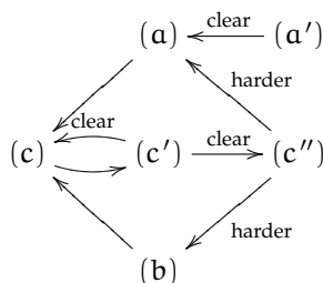
FIGURE 16.1. Structure of the proof of Theorem 16.2.2, up to the last step
