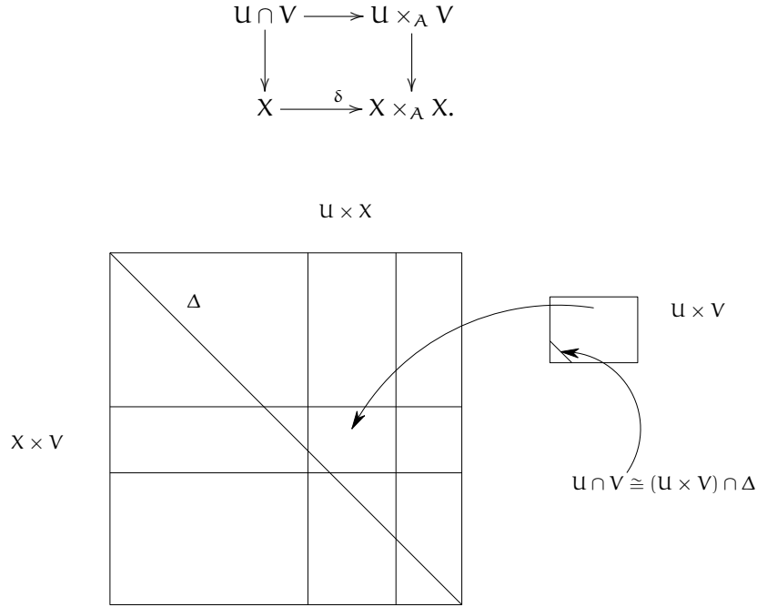
FIGURE 11.3. \Delta \cap (U \times_A V) \cong U \cap V (Exercise 11.3.M)
