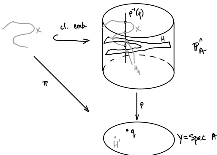
FIGURE 18.1. The key construction in the proof of Theorem 18.1.6
