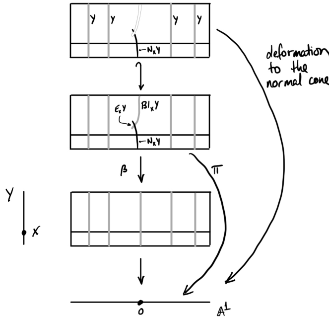
FIGURE 22.3. Deformation to the normal cone (§22.4.17)
