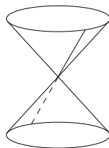
FIGURE 13.1. V(x, z) \subset \operatorname{Spec} k[x, y, z]/(xy - z^2) is a line on a cone
