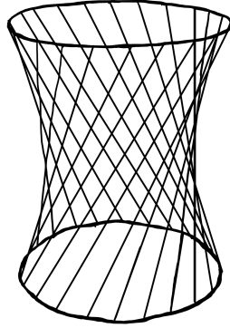
FIGURE 9.2. One of the two rulings on the quadric surface V(wz - xy) \subset \mathbb{P}^3 . One ruling contains the line V(w, x) , and the other contains the line V(w, y) .
