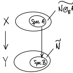
FIGURE 14.1. The pullback of a quasicoherent sheaf (module-theoretically)
