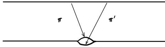
FIGURE 11.4. Two different maps to a nonseparated scheme agreeing on a dense open set (see Exercise 11.4.D)
