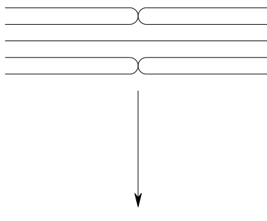
FIGURE 21.4. An example where the branch divisor appears with multiplicity 2 (see Exercise 21.4.C)
