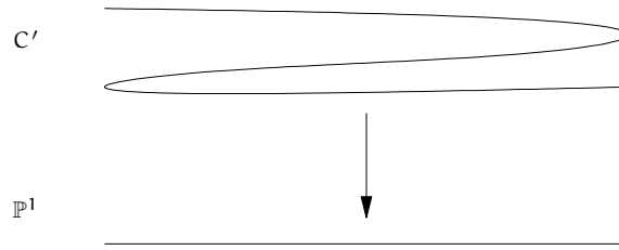
FIGURE 16.3. Constructing a projective regular model of a curve C over k via a finite cover of \mathbb{P}^1
