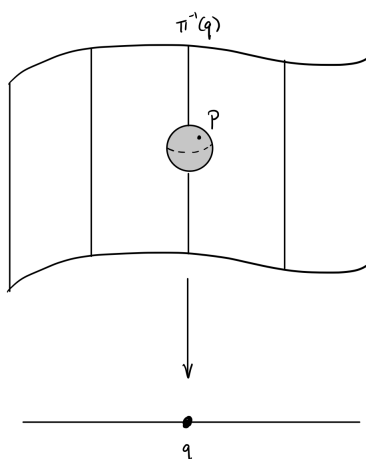
FIGURE 12.4. Exercise 12.4.A: the codimension of a point in the total space is bounded by the sum of the codimension of the point in the fiber plus the codimension of the image in the target
