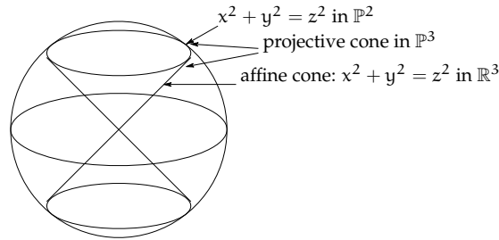
FIGURE 4.9. The affine and projective cone of x^2 + y^2 = z^2 in classical geometry
