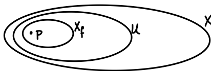
FIGURE 16.2. Visual aid for the proof of Theorem 16.2.2
