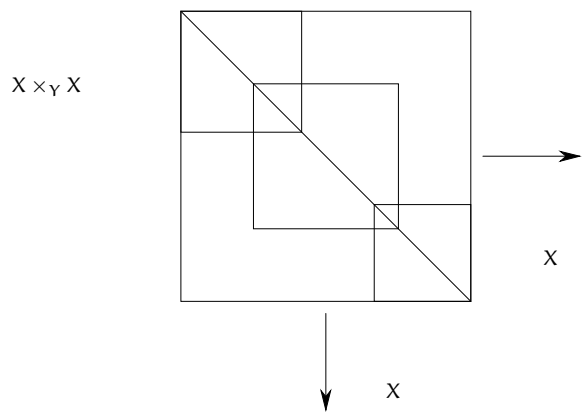
FIGURE 10.1. A neighborhood of the diagonal is covered by \cup_{ij} \times_{v_i} U_{ij}
