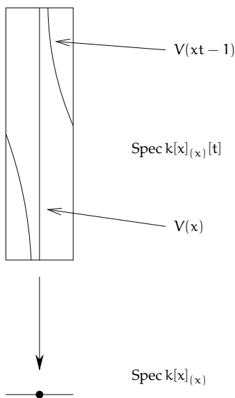
FIGURE 11.2. Dimension and codimension behave oddly on the surface \text{Spec } k[x]_{(x)}[t]
