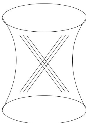
FIGURE 8.3. The two rulings on the quadric surface V(wz - xy) \subset \mathbb{P}^3 . One ruling contains the line V(w, x) and the other contains the line V(w, y) .
