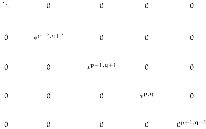
FIGURE 1.1. A (p, q) -strip (in S^{p, q} \subset E^{p+q} ). Clearly S^{0, k} = E^k .
