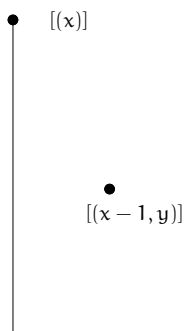
FIGURE 3.10. The set S of Exercise/example 3.7.A, pictured as a subset of \mathbb{A}^2
