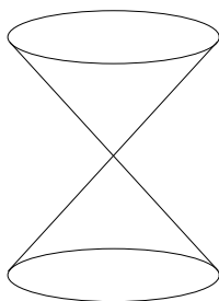
FIGURE 8.2. The cone \text{Spec } k[x, y, z]/(z^2 - x^2 - y^2) .
