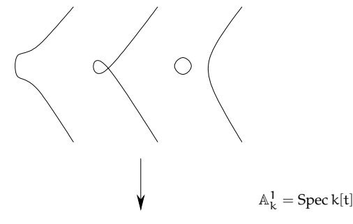
FIGURE 24.1. A flat family of smooth curves degenerating to a nodal curve: y^2 = x^3 - tx^2 .
