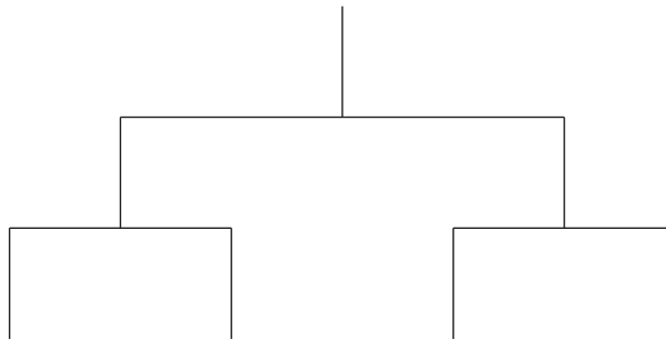
Figure 7: Dendrogram
