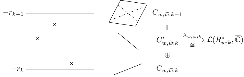
FIGURE 5.2. Illustration of the spaces C_{w, \tilde{w}; k} and C'_{w, \tilde{w}; k} in Lemma 5.18; the crosses indicate resonances, the total rank of which in the displayed strip is equal to D'_k .
