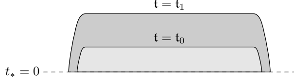
FIGURE 8.10. Illustration of the energy estimate (8.34), with u vanishing in t_* < 0 . The norm of \mathcal{P}_h u is taken on the union of the shaded regions, and we obtain control of u on the lightly shaded region.
