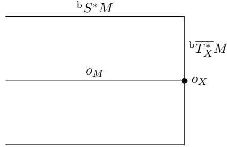
FIGURE A.1. The radially compactified cotangent bundle {}^b\overline{T^*M} near {}^b\overline{T^*_X M} ; the cosphere bundle {}^bS^*M , viewed as the boundary at fiber infinity of {}^b\overline{T^*M} , is also shown, as well as the zero section o_M \subset {}^b\overline{T^*M} and the zero section over the boundary o_X \subset {}^b\overline{T^*_X M} .
