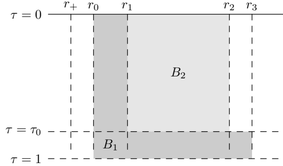
FIGURE 8.12. Illustration of the energy estimate (8.43) beyond the cosmological horizon r = r_+ . The norm of \mathcal{P}_h u is taken on r^{-1}([r_0, r_3]) \cap \tau^{-1}([0, 1]) , and we obtain control of u on the lightly shaded region, assuming a priori control on the dark region.
