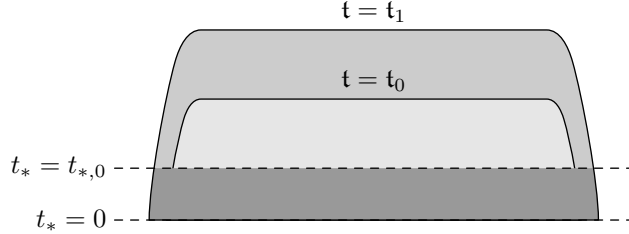
FIGURE 8.11. Illustration of the energy estimate (8.35). The norm of \mathcal{P}_h u is taken on the union of the shaded regions, and we obtain control of u on the lightly shaded region, assuming a priori control on the dark region.
