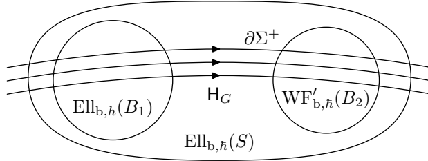
FIGURE 8.3. Propagation of regularity in the future direction within \partial\Sigma^+ : We can propagate microlocal control from \text{Ell}_{b,\hbar}(B_1) to \text{Ell}_{b,\hbar}(B_2) . In \partial\Sigma^- , the arrows are reversed, corresponding to propagation in the backwards direction along H_G (which is still the future direction in \partial\Sigma ).
