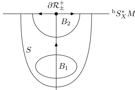
FIGURE 8.4. Propagation of singularities near a component \partial\mathcal{R}_\pm^\pm of the radial set within \partial\Sigma^+ : We can propagate microlocal control from \text{Ell}_{b,\hbar}(B_1) to \text{Ell}_{b,\hbar}(B_2) , in particular into the boundary, along the forward direction of the H_G -flow. In \partial\Sigma^- , we can propagate into the boundary as well by propagating backwards along the H_G -flow.
