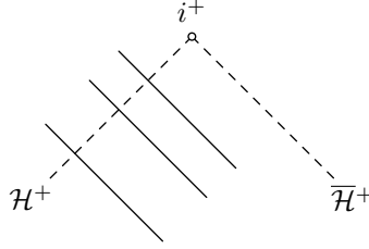
FIGURE 7.1. Level sets of u for which (u, v = r) gives coordinates near the event horizon, away from the cosmological horizon, in which the Schwarzschild–de Sitter metric takes the form (7.9). Analogous coordinates can be chosen near the cosmological horizon, away from the event horizon.
