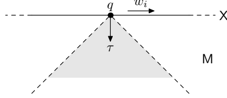
FIGURE C.1. A neighborhood of a point q on the conformal boundary of de Sitter space; also indicated (shaded) is the static model at q , which near q is the interior of the backward light cone from q with respect to \bar{g} (and thus g ).
