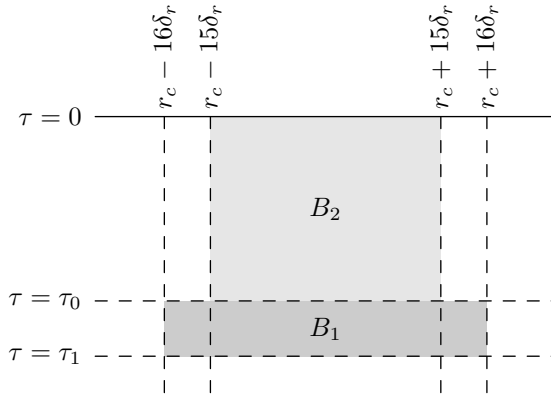
FIGURE 8.8. Propagation near the zero section in the vicinity of the critical set of \nabla t_* : Control on the elliptic set of B_1 propagates to the elliptic set of B_2 .
